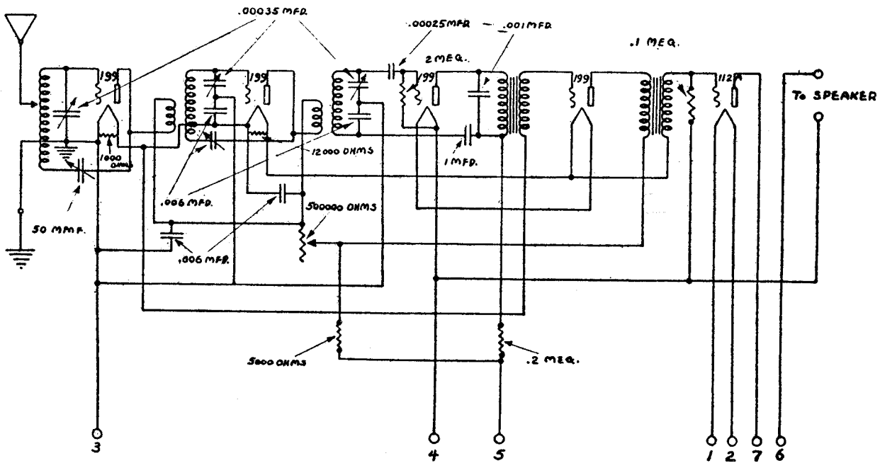
Model 115-BO (1926)
